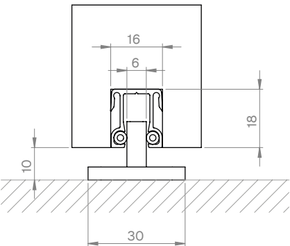
Lower guide profile
