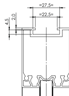
Housing seat for aluminium bracket profile
