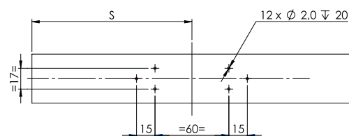
Fixing hole pattern
