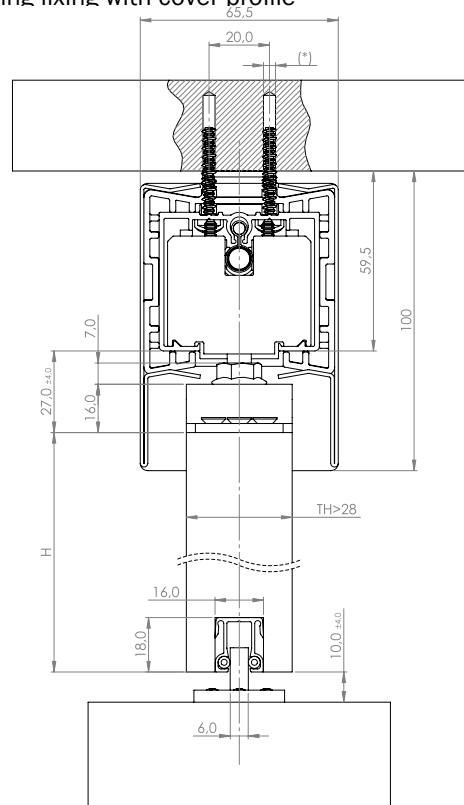
Ceiling fixing with cover profile
