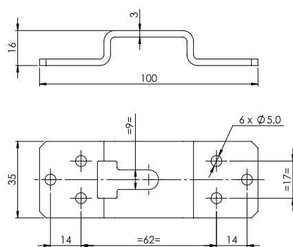
Standard bracket dimensions
