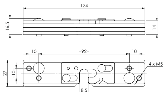
Aluminium-version bracket dimensions
