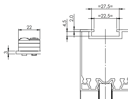
Housing seat for aluminium bracket profile
