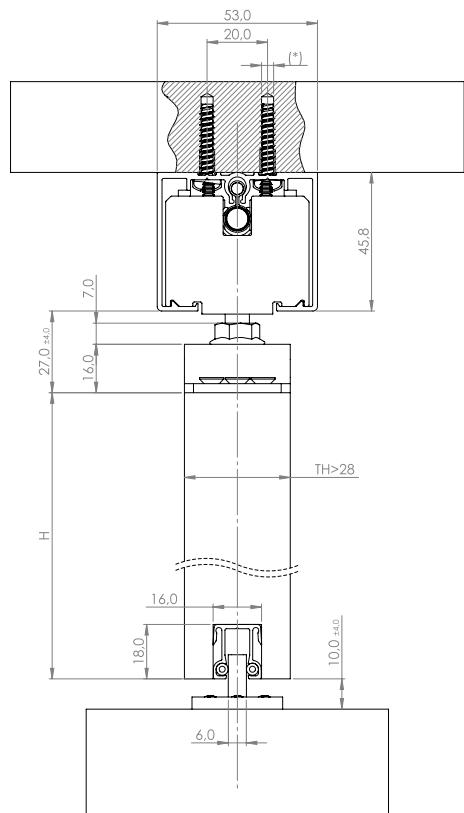
Ceiling fixing
