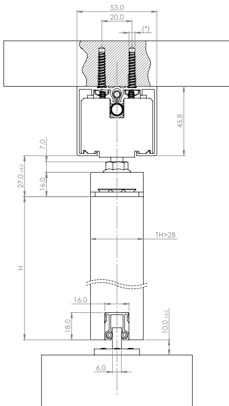
Ceiling fixing
